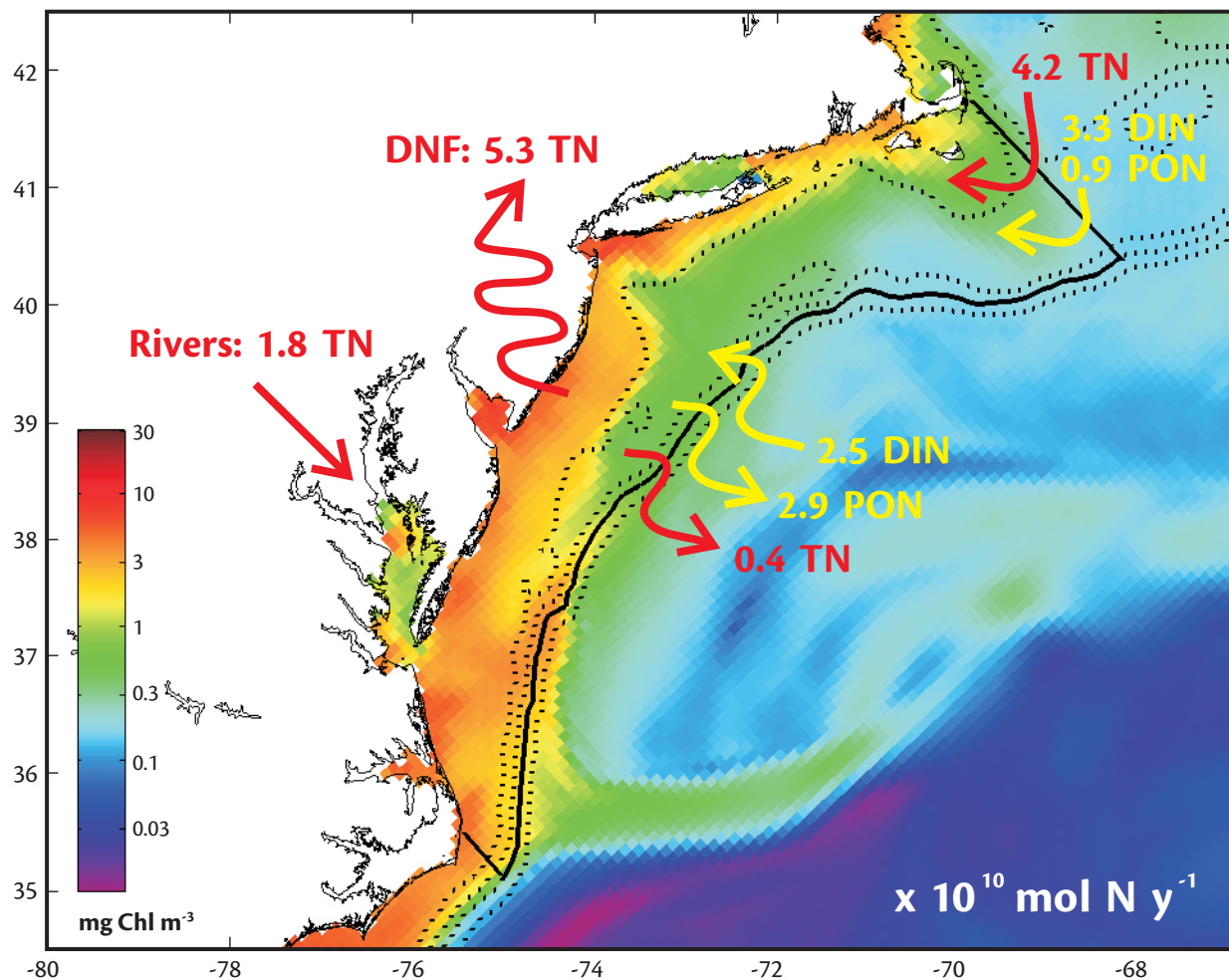
Figure 9. Model-predicted mean surface chlorophyll for July 1994 in the Middle Atlantic Bight (MAB) overlain by a model-derived nitrogen budget for the MAB shelf region. The annual mean nitrogen budget for the MAB shelf region (indicated by the solid black lines) was derived by diagnosing the fluxes of total nitrogen (TN, red numbers and arrows), dissolved inorganic nitrogen (DIN, yellow) and particulate organic nitrogen (PON, yellow) across two cross-shelf transects at Cape Cod and Cape Hatteras and across the 200 m isobath (the 40, 100, 200, and 500 m isobaths are indicated by dotted black lines) in addition to the annual river input and the denitrification (DNF) loss.
