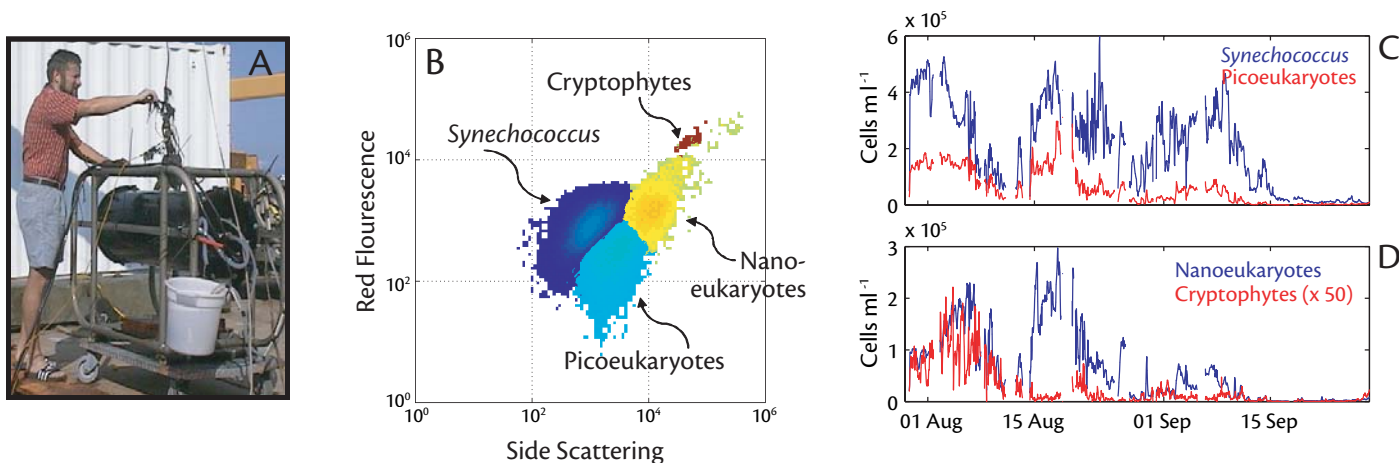
Figure 2. FlowCytobot (A), an automated submersible flow cytometer designed and built at the Woods Hole Oceanographic Institution (Olson et al., 2003), has been successfully deployed at coastal cabled observatory sites on the U.S. East Coast. FlowCytobot makes nearly continuous measurements of pico/nanophytoplankton abundance, cell scattering, and cell fluorescence characteristics (B, typical data from 1 hour of sampling; classification of cells considers all measured properties including orange fluorescence, critical for discrimination of Synechococcus and cryptophytes). A two-month deployment at the Long-Term Environmental Observatory off New Jersey in 2001 reveals a high level of temporal variability in abundance of Synechococcus , cryptophytes and other pico- and nanophytoplankton (C, D), some of which can be explained on the basis of changes in population growth rates inferred from FlowCytobot-based observations of diel changes in cell size distributions (Sosik et al., 2003). An autonomous flow cytometer is now commercially available in portable, floating, and submersible versions (CytoBuoy b.v., The Netherlands; http://www.cytobuoy.com ).
