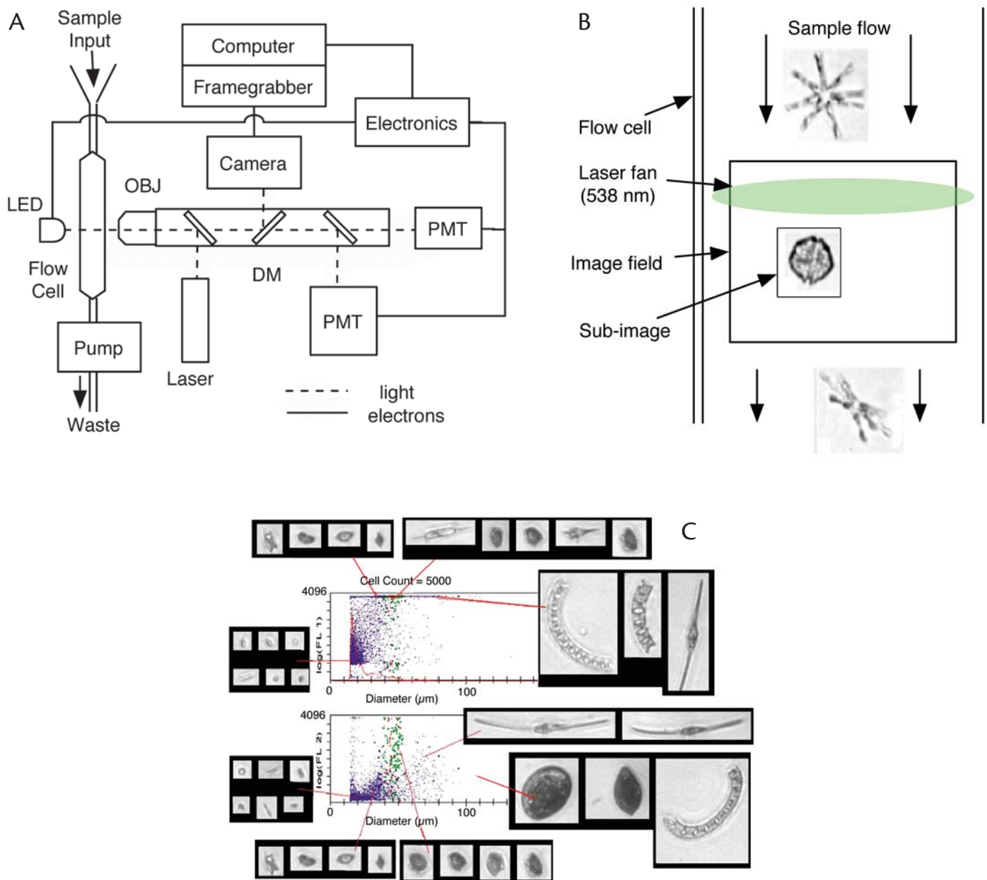
Figure 1. Schematic diagrams and results from the FlowCAM imaging-in-flow system (Fluid Imaging Technologies, USA; www.fluidimaging.com ). Sample fluid is pulled through the flow cell at rates up to 4 mL/min. (A) When a cell enters the field of view, fluorescence is excited by a fan of laser light. Epifluorescence optics are used that employ dichroic mirrors (DM) to split the light signals. Different objectives (OBJ) can be used for different magnifications (e.g., 4X to 20X). The fluorescence signal is detected by photomultiplier tubes (PMT) and triggers a light emitting diode (LED) to flash and backlight the flow cell. The camera image is digitized by the frame grabber. The cell is located within the image and measured, and a subimage is stored on disk in real time. Particles can also be detected by light scatter (detector not shown for simplicity). (B) Details of the field of view of the flow cell. (C) These images are linked to the size and fluorescence values and results can be browsed using the interactive scattergram. The dot plot shows fluorescence versus size and populations can be investigated by selecting points and the corresponding images are displayed.
