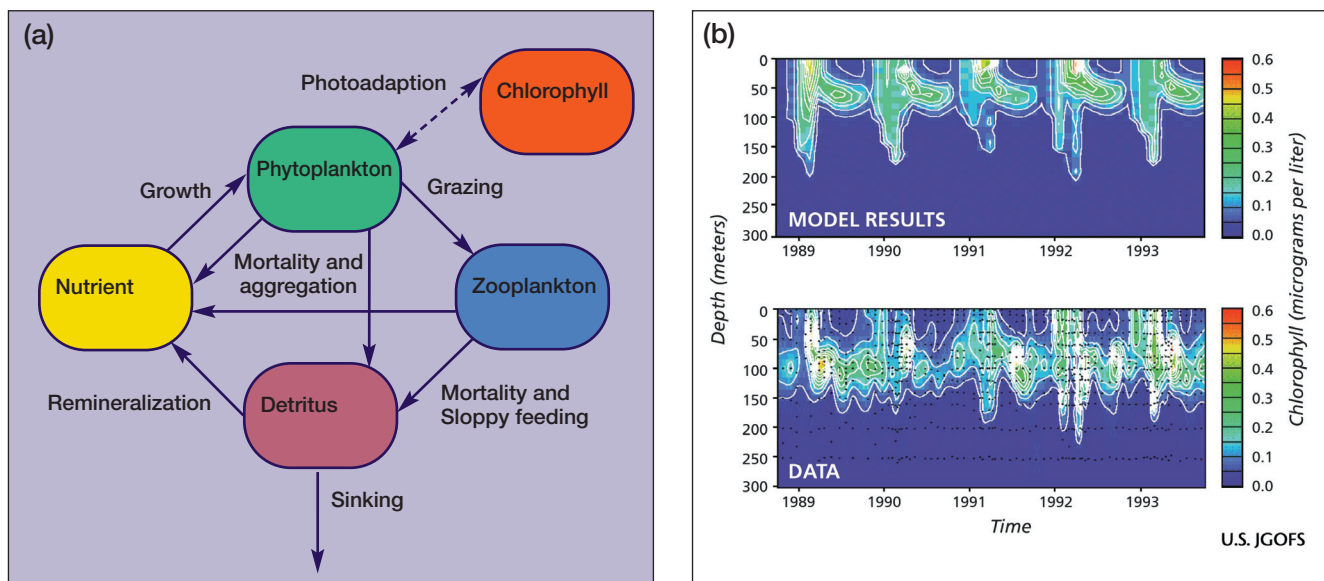
Figure 4. (a) Schematic of a simple marine ecosystem model with separate compartments for nutrients, phytoplankton, zooplankton, detritus (collectively NPZD), and chlorophyll. (b) Depth-versus-time comparison of observed and simulated chlorophyll concentrations from a 1-D version of the model applied to a multi-year record from the Bermuda Atlantic Time-series Study (BATS) site in the Sargasso Sea. Deep convection in the winter brings nutrients to the surface, generating a winter/spring phytoplankton bloom. During the summer, biological export drives surface nutrients and chlorophyll to very low levels. A subsurface, deep chlorophyll maximum forms where light from above and nutrients from below are both available.
